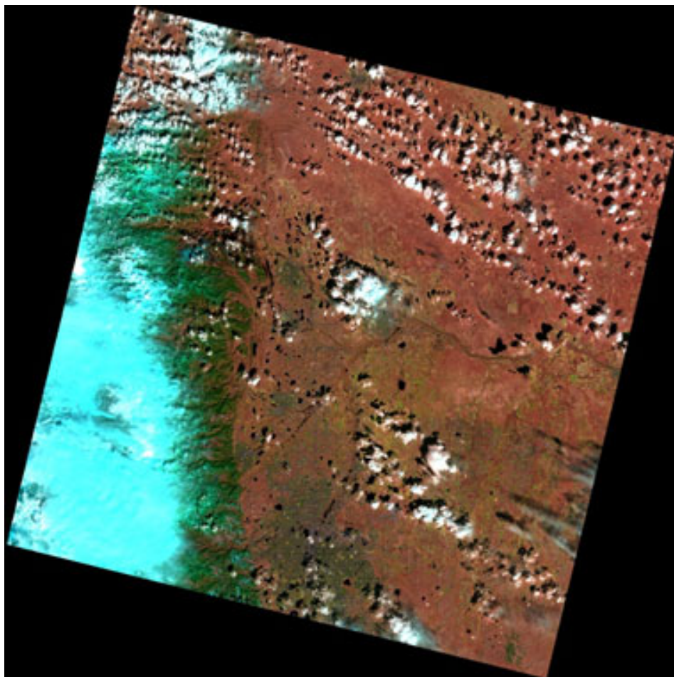
LDCM image acquired March 18, 2013, displayed in Bands 6,5,4 and sharpened with panchromatic band 8.
