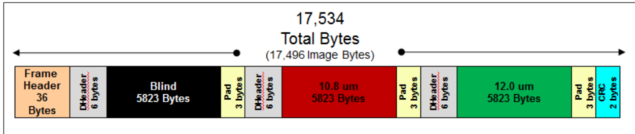
Figure 3-9. TIRS Band Output Order
